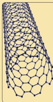
Carbon Nanotube
